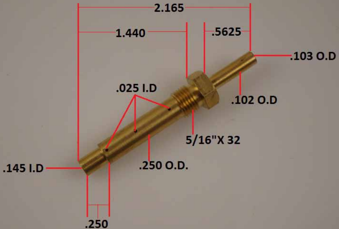
ABC1156 Main Nozzle
